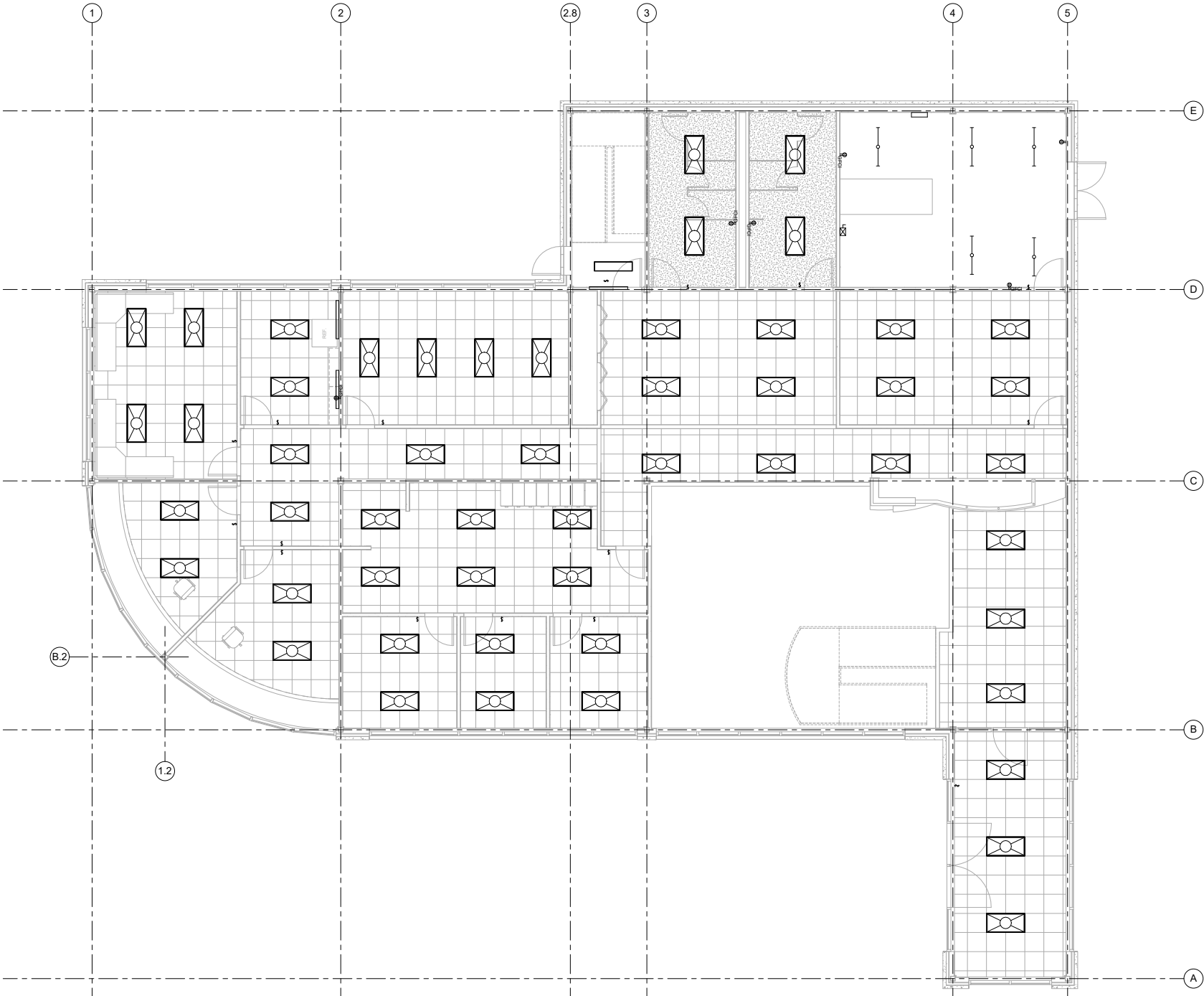
Level 1 - Ceiling Plan
